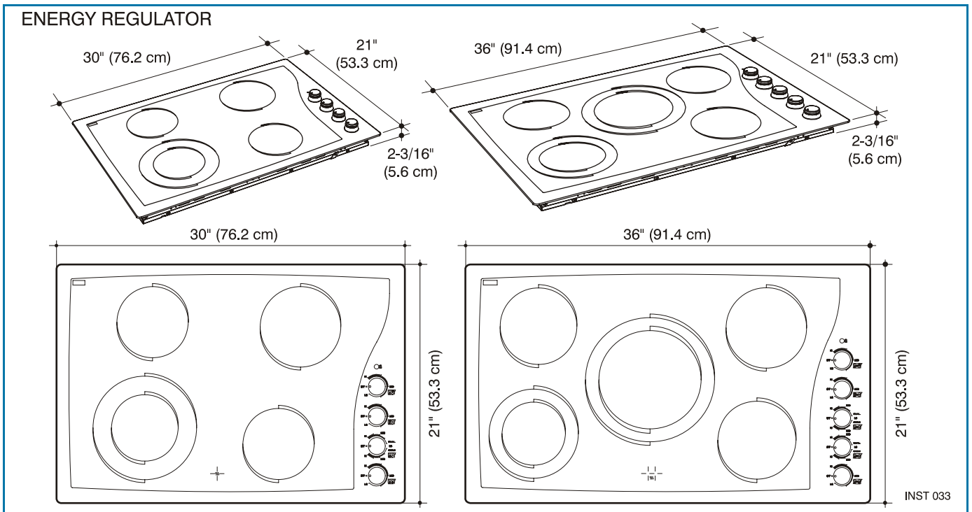
Figure 2. Energy regulator
